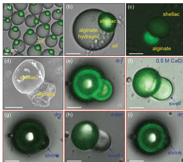
Figure 3. Hydration and dehydration of the alginate bulb showing typical hydrogel features. (a,b) Overlays of confocal fluorescent (green) and optical (gray) images of hydrogel–solid particles made with FITC-labeled alginate. The fluorescence observed in the shellac bulb indicates that some alginate is dragged into the shellac when it precipitates. The hydrogel bulb shows only a very weak fluorescent intensity due to the low concentration of alginate in water. (c) When the particle is dried, the alginate bulb shows a fluorescence much stronger than that of shellac, and the whole particle attains a mushroom-like shape. (d) SEM image of an amphiphilic particle made with FITC-labeled alginate. (e–i) Cross-linking of alginate hydrogel bulbs using \text{Ca}^{2+} cations forms a stable amphiphilic hydrogel–solid particle. The alginate bulb shows typical features of a hydrogel in that it swells when it is submerged in water and shrinks when it is dry. During the hydration and dehydration processes, the configuration of the particle has changed and the alginate bulb is no longer in the focal plane, thus showing a low fluorescent intensity even when it is dehydrated. (e–i) Images of the same particle. The scale bar is 10\ \mu\text{m} in all images.
